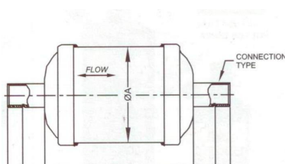
DCH BI-FLOW DRIER WITH ODS CONNECTION DIMENSIONS
