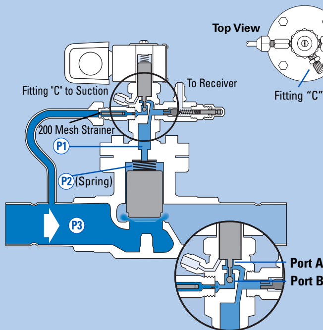
Figure 5 Coil De-Energized Differential Operation
