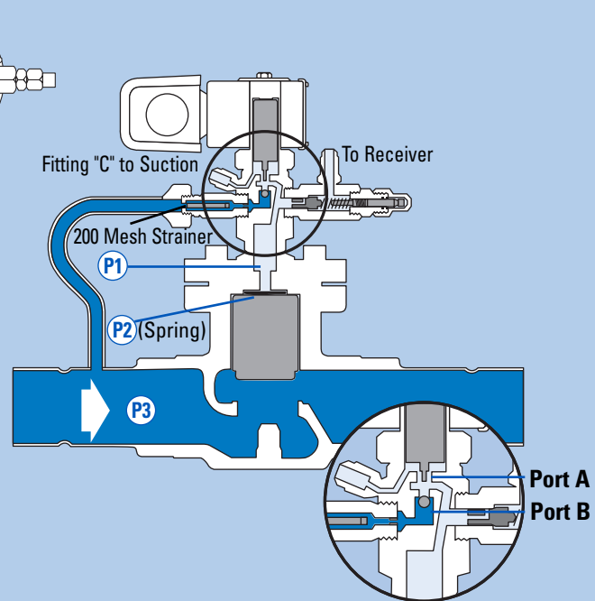
Figure 6 Coil Energized Full Open Operation
