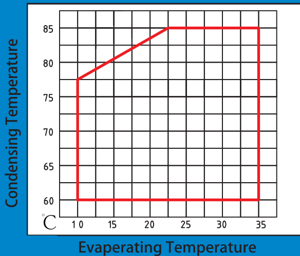
R134a Application Limits
