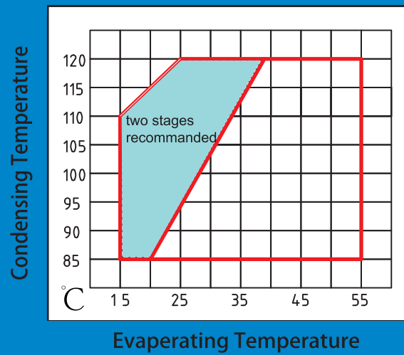
R245fa Application Limits
